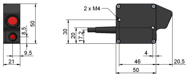
LAM-S-20 LAM-F-20
